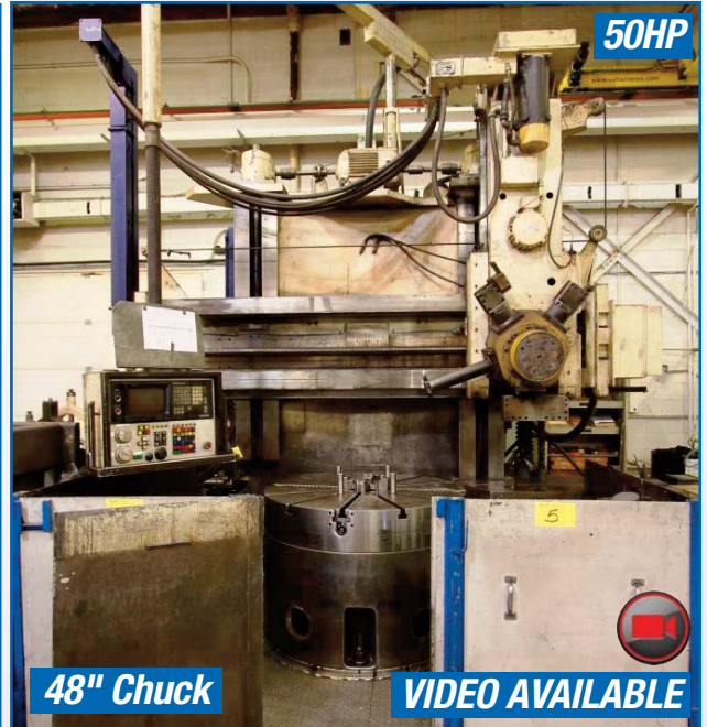
GIDDINGS & LEWIS TYPE 48" VTL VERTICAL TURNING LATHE
